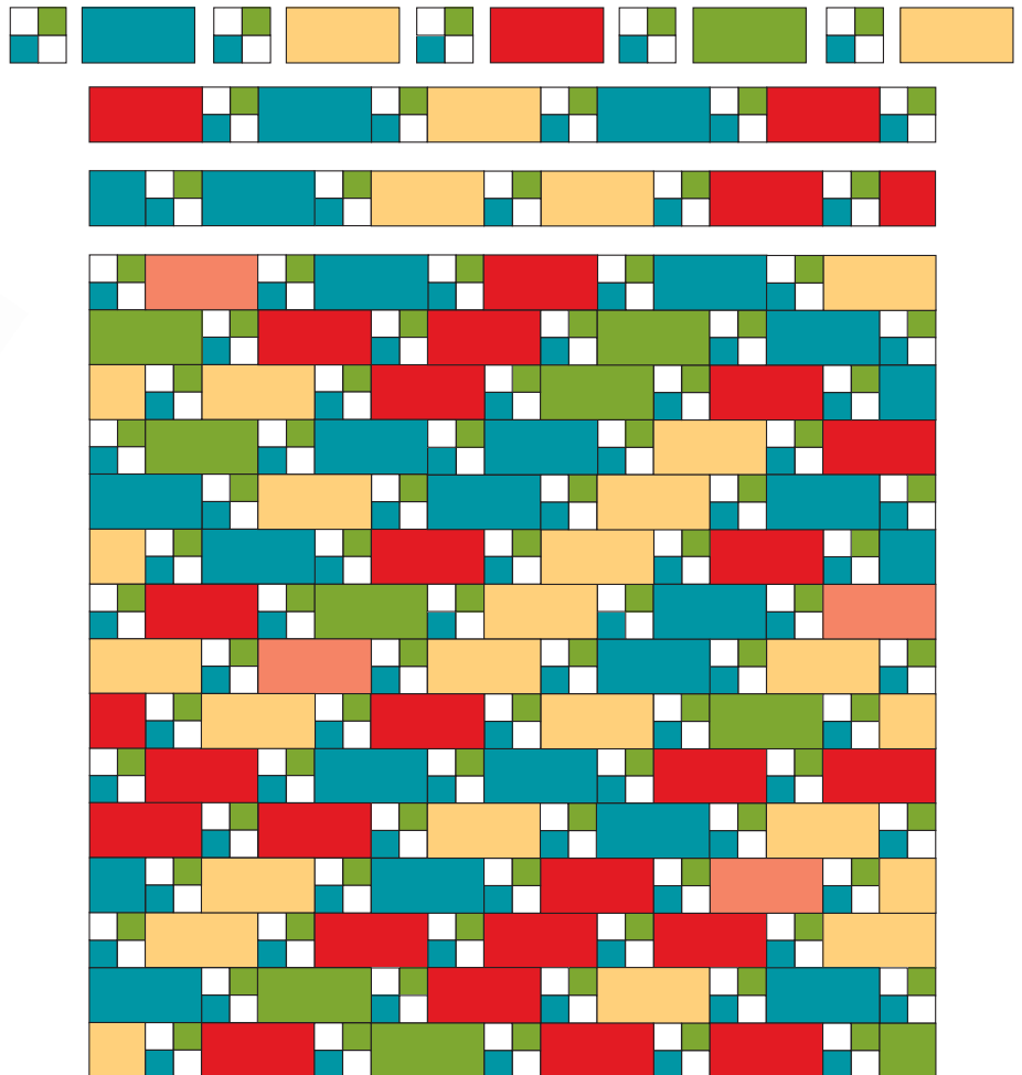
Quilt Diagram
